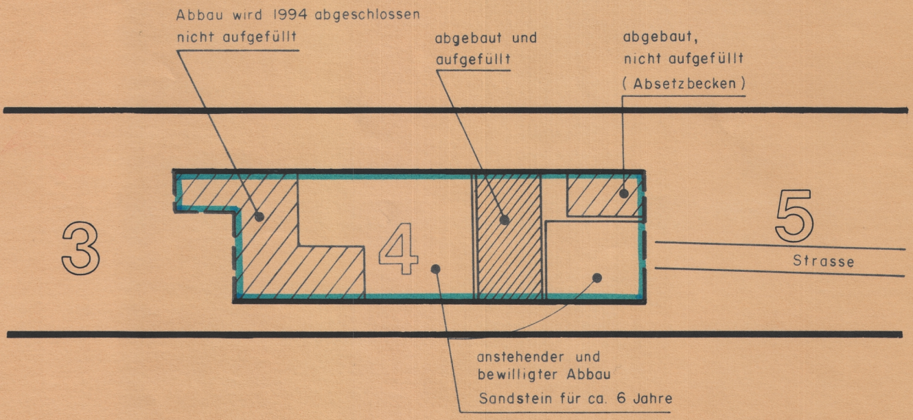
DETAIL A 1:1000
